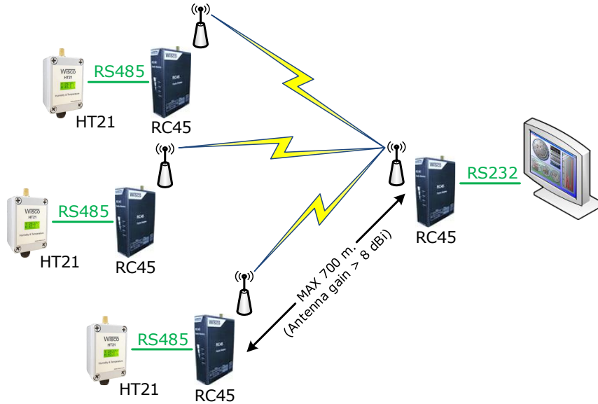
Connection via Wireless (Point to Multipoint)
